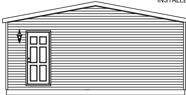
LEFT ELEVATION
