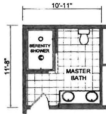
OPTIONAL SERENITY SHOWER N/A W/OPTIONAL END ENTRY
