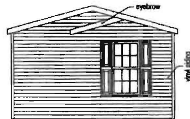
SINGLE WIDE ELEVATION "S9" SINGLE WIDE EYEBROW ELEVATION EYEBROW (DOESNT INCLUDE SHUTTERS) 150 S.F.
