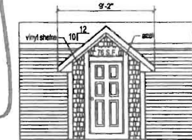
9' HUD DORMER "S7" 6" DROP EAVE DORMER 7' FAUX BUMPOUT AZEK TRIM/SHAKE
