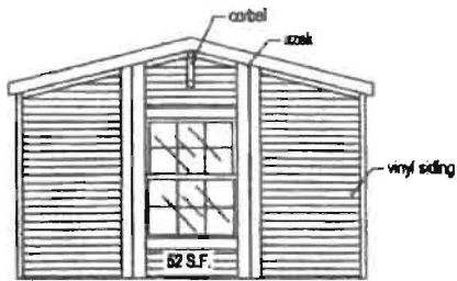
SINGLE WIDE ELEVATION "S1" AZEK TRIM & CORBEL (DOESNT INCLUDE 46" WINDOW) 150 S.F.
