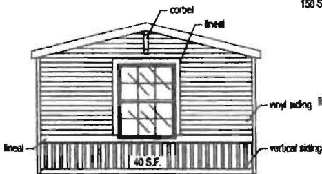
SINGLE WIDE ELEVATION "S4" VERTICAL SIDING, CORBEL, LINEALS (DOESNT INCLUDE 46" WINDOW) 150 S.F.
